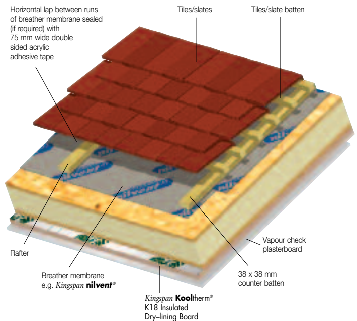
Figure 18 37.5 mm Kingspan Kooltherm® K18 Insulated Plasterboard. Non tenting breather membrane (e.g. Kingspan nilvent® ), 38 mm x 38 mm vertical treated timber counter battens, tiling battens and tiles / slates. U-value 0.16 W/m 2 ·K.
