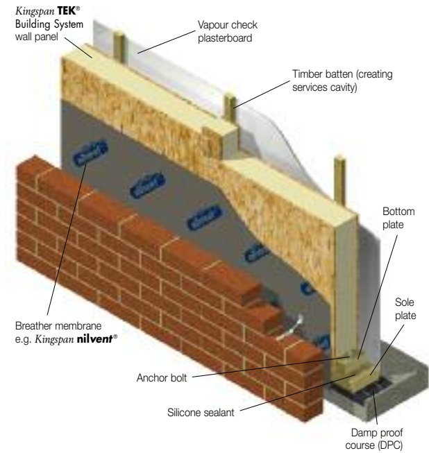
Figure 11 12.5 mm vapour check* plasterboard on 25 mm timber battens † . Non tenting breather membrane (e.g. Kingspan nilvent®, 50 mm cavity, brickwork facing. U-value 0.19 - 0.21 W/m 2 ·K.
