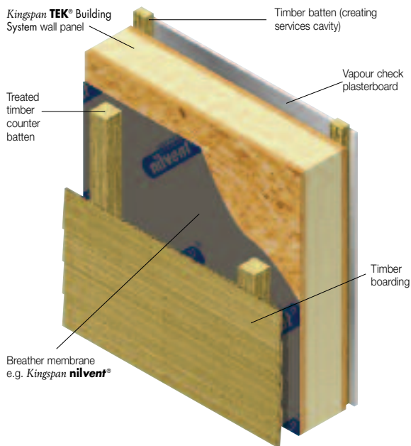
Figure 15 12.5 mm vapour check* plasterboard on 25 mm timber battens†. Non tenting breather membrane (e.g. Kingspan nilvent® , 25 mm (min.) vertical treated timber counter battens, timber boarding. U-value 0.20 - 0.22 W/m 2 ·K.
