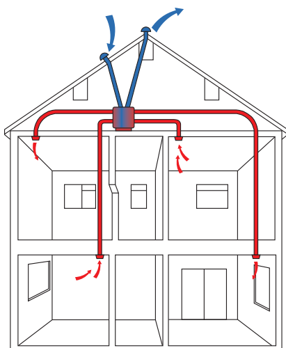
Figure 1 MVHR System
