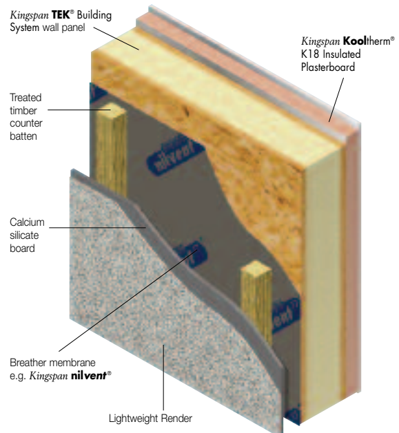
Figure 14 Kingspan Kooltherm® K18 Insulated Plasterboard. Non tenting breather membrane (e.g. Kingspan nilvent®, 25 mm (min.) vertical treated timber counter battens, calcium silicate board with lightweight render coating.
