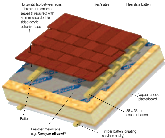
Figure 17 12.5 mm vapour check* plasterboard on 25 mm timber battens†. Non tenting breather membrane (e.g. Kingspan nilvent® ), 38 mm x 38 mm vertical treated timber counter battens, tiling battens and tiles / slates. U-value 0.18 - 0.20 W/m 2 ·K.
