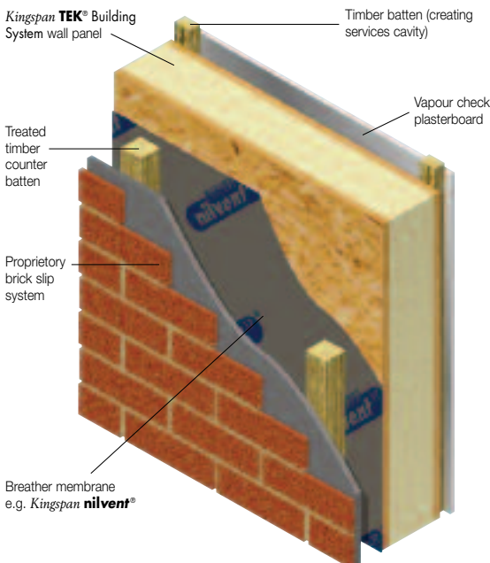
Figure 13 12.5 mm vapour check* plasterboard on 25 mm timber battens † . Non tenting breather membrane (e.g. Kingspan nilvent®, 25 mm (min.) vertical treated timber counter battens, proprietary brick slip system. U-value 0.20 - 0.22 W/m 2 ·K.
