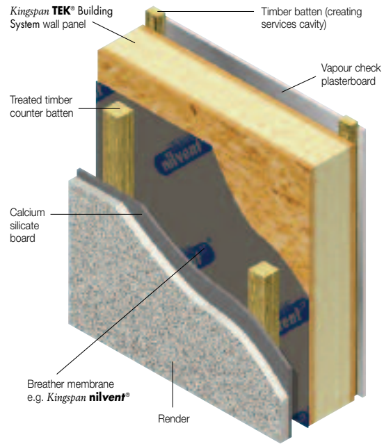
Figure 12 12.5 mm vapour check* plasterboard on 25 mm timber battens † . Non tenting breather membrane (e.g. Kingspan nilvent®, 25 mm (min.) vertical treated timber counter battens, calcium silicate board with lightweight render coating. U-value 0.20 - 0.22 W/m 2 ·K.
